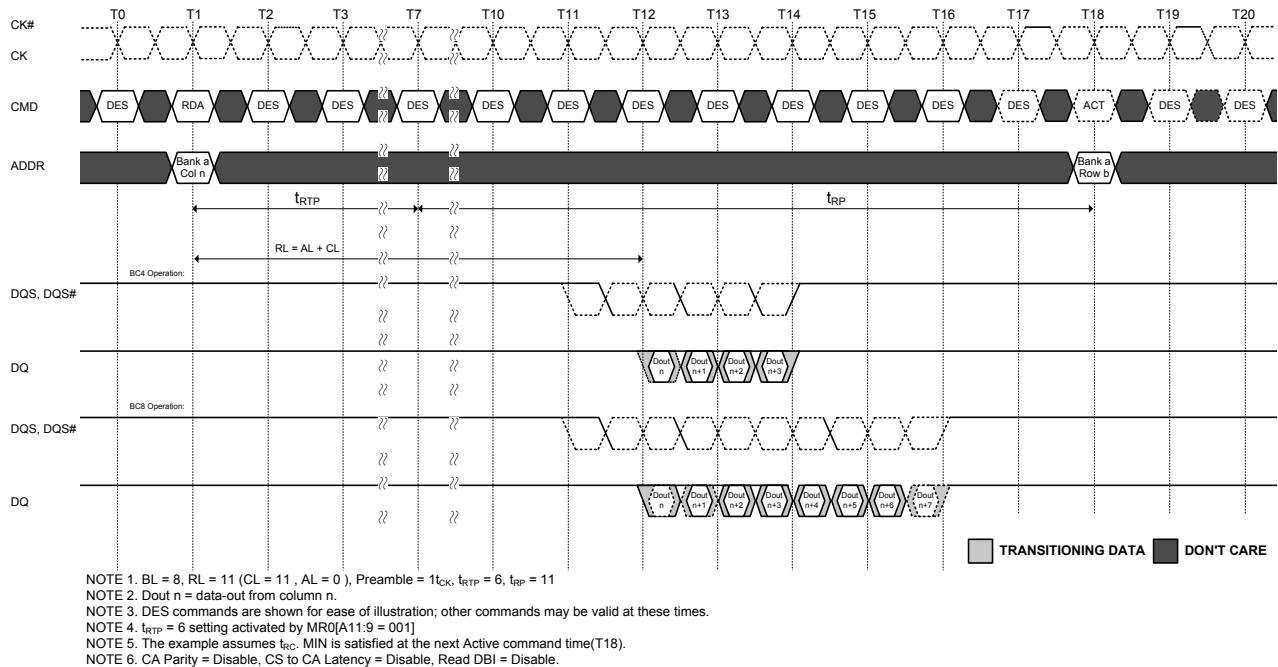
Figure 120. READ with Auto Precharge and 1t_{CK} Preamble
